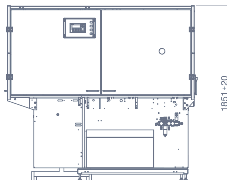
HL configuration
