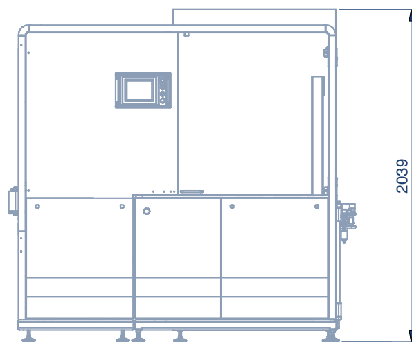
DIL/LIL configuration
